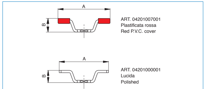
Farfalla in acciaio inox - Stainless steel butterfly handle - Papillon en acier inox - Flügelgriff aus Edelstahl - Mariposa en acero inox.
